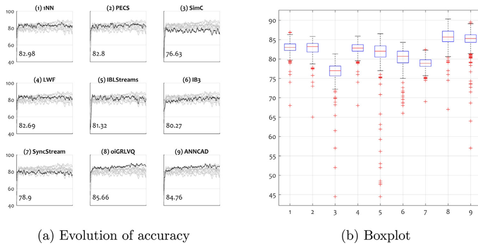
Fig. 3. Hyperplane generator: accuracy (in %) of the algorithms without concept drift. The evolution of the accuracy statistic is shown in subfigure (a), and the distribution of the instantaneous accuracy values for each algorithm is shown by a boxplot in subfigure (b). The average accuracy is shown in the bottom-left corner of each sub-plot in (a).
