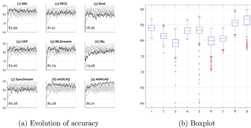
Fig. 6. Random tree generator: accuracy (in %) of the algorithms without concept drift. The average accuracy is shown in the bottom-left corner of each sub-plot in (a).
