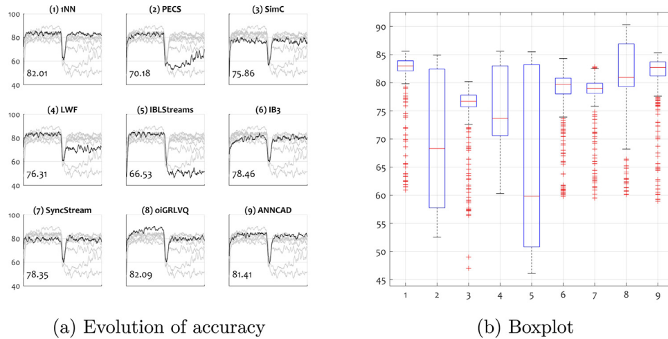
Fig. 4. Hyperplane generator: accuracy (in %) of the algorithms with gradual concept drift. The average accuracy is shown in the bottom-left corner of each sub-plot in (a).
