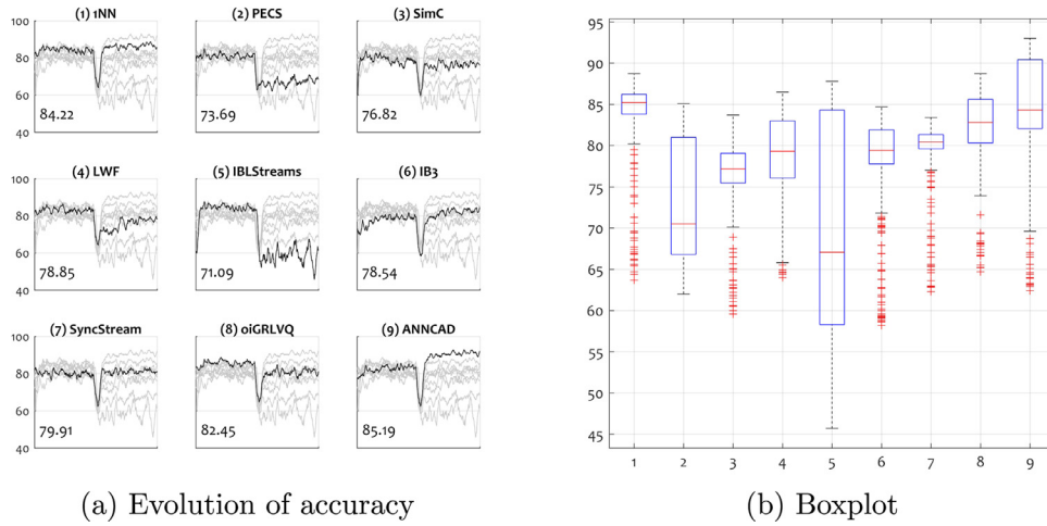
Fig. 7. Random tree generator: accuracy (in %) of the algorithms with gradual concept drift. The average accuracy is shown in the bottom-left corner of each sub-plot in (a).
