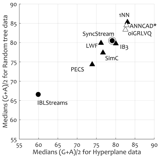
Fig. 9. Scatterplot of the 9 methods in the space of median accuracies for the two synthetic data sets without noise. The significance of the markers is as follows: shape indicates whether or not the method uses explicit change detection: circle \circ – yes, triangle \triangle – no; and a filled shape indicates a prototype selection method while an empty shape indicates a prototype generation method. The filled marker for SyncStream is circled to indicate that this method belongs to both the prototype selection and prototype generation categories. The ensemble approach, ANNCAD, is indicated with an asterisk.
