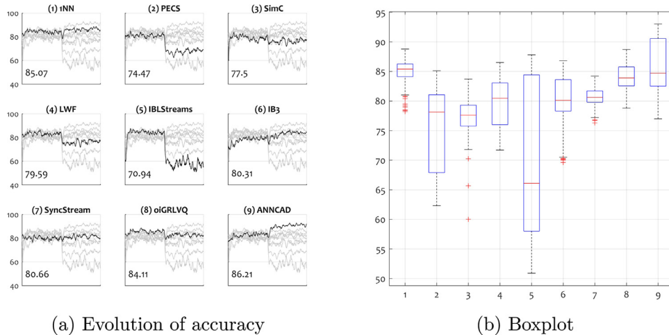
Fig. 8. Random tree generator: accuracy (in %) of the algorithms with abrupt concept drift. The average accuracy is shown in the bottom-left corner of each sub-plot in (a).
