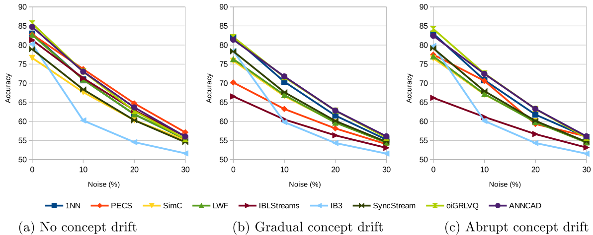
Fig. 10. Accuracy of the different classifiers with and without noise on the hyperplane generator.
