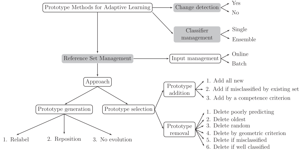
Fig. 2. A taxonomy of nearest-neighbour methods for streaming data. The nodes in boxes show properties that should be specified, and their values are chosen among the leaves of the respective sub-tree. Shaded boxes are areas for which algorithms might be developed independently. For example, an ensembling method might be developed which is agnostic regarding the base classifier; the base classifier could then be any classifier trained on the chosen reference set.
