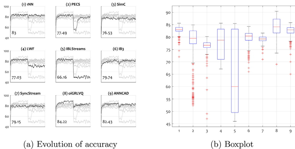
Fig. 5. Hyperplane generator: accuracy (in %) of the algorithms with abrupt concept drift. The average accuracy is shown in the bottom-left corner of each sub-plot in (a).
